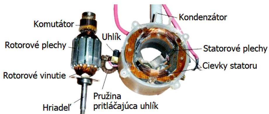
Stator
